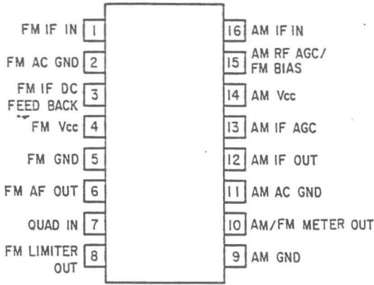
IC1 K84419A
